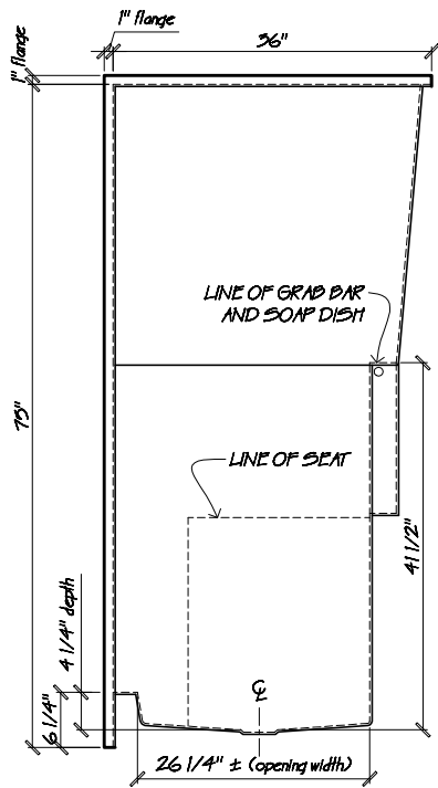
RIGHT END VIEW scale: 1/2" = 1"
