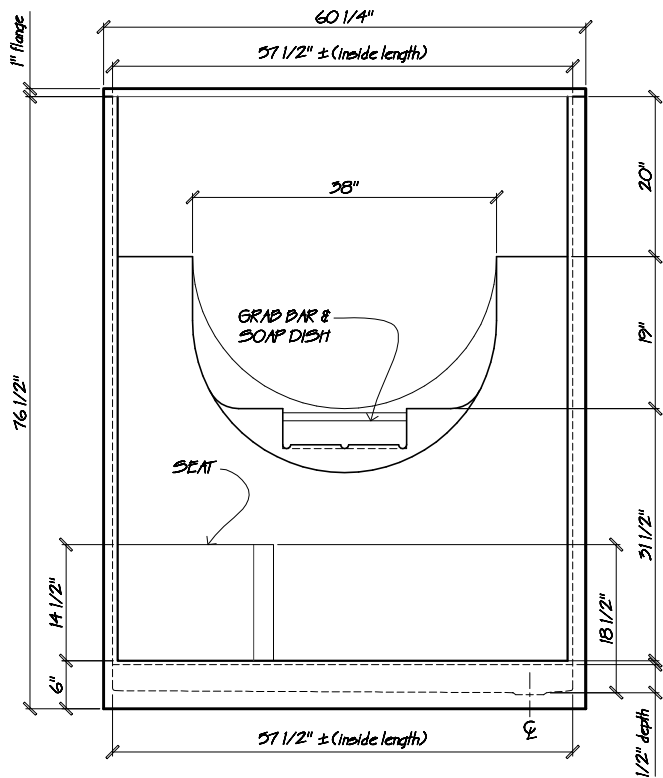
FRONT VIEW scale: 1/2" = 1"
