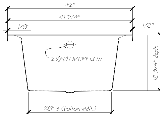
END VIEW
