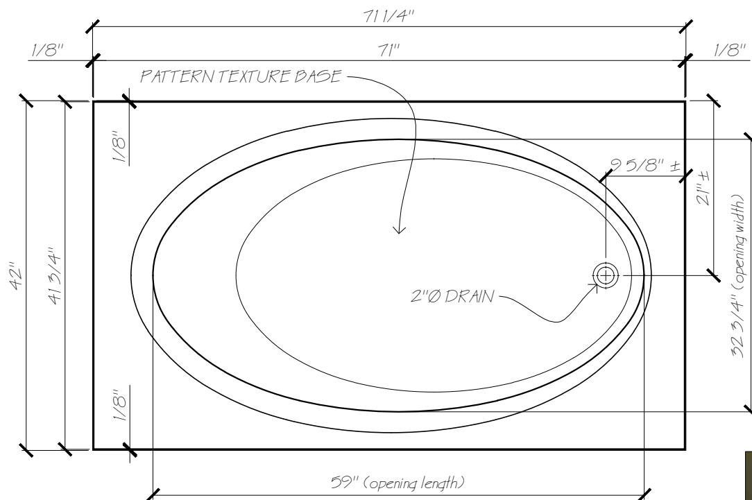
PLAN VIEW
