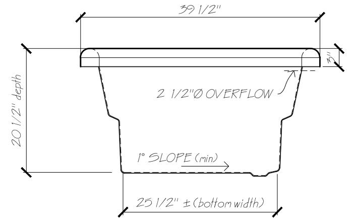
END VIEW
