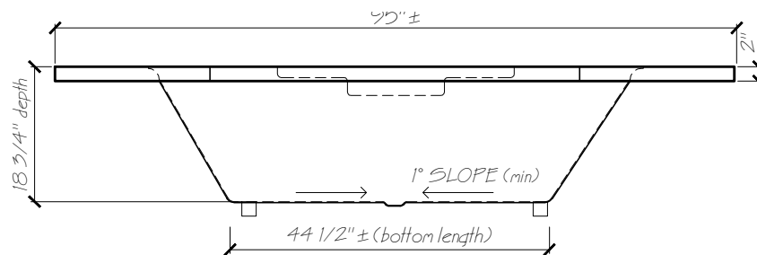
FRONT VIEW
