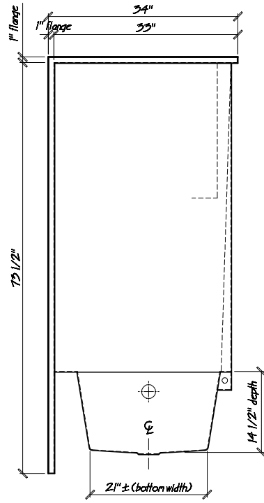
RIGHT END VIEW
