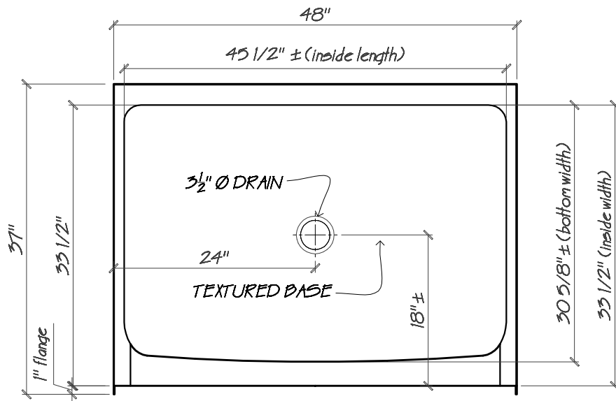
PLAN VIEW scale: 3/4" = 1"
