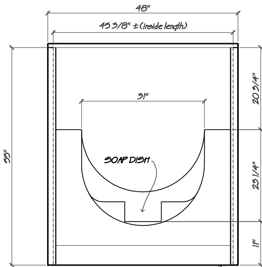
LINE OF ATTACHMENT SEE RSD 4836CS (fixed w/ \frac{1}{4}'' \varnothing bolt & nut & flange)
